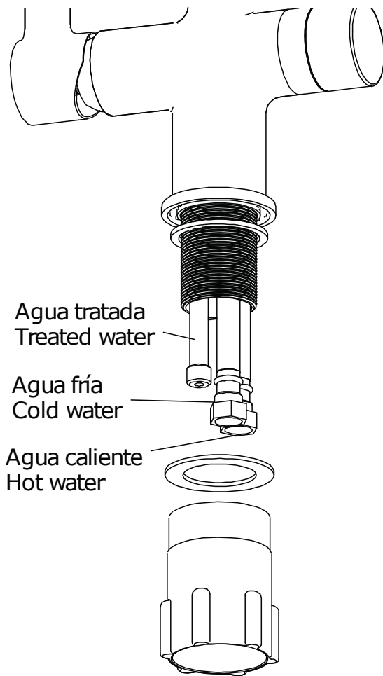
Salida de agua tratada / Treated water outlet
